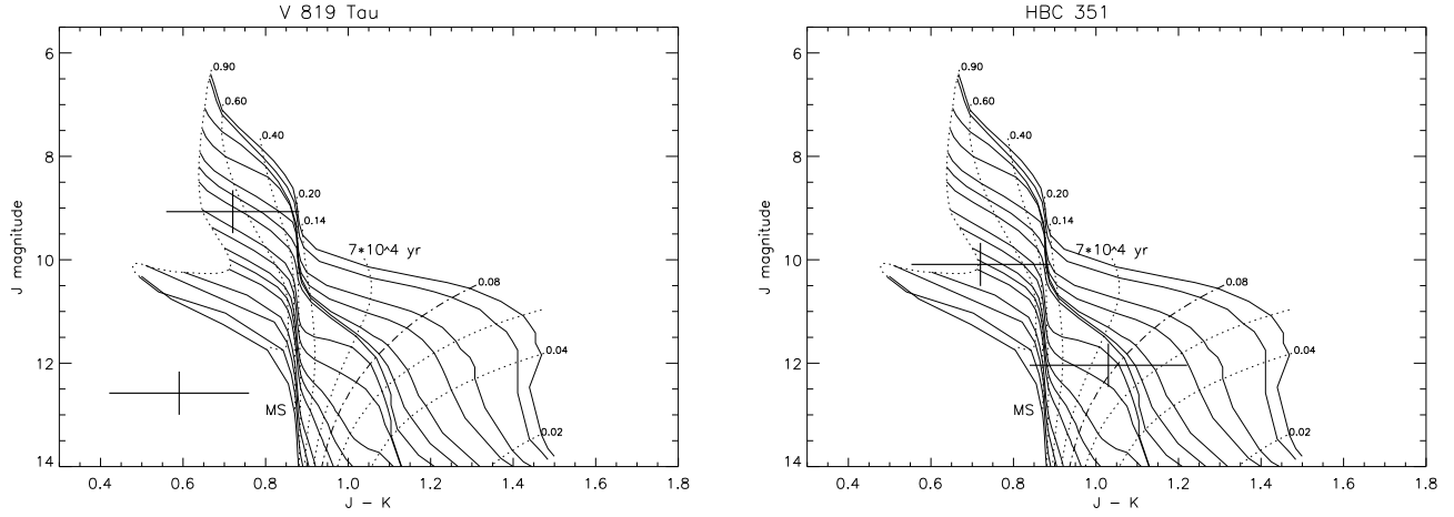
Fig. 4. Examples of colour-magnitude diagrams for two WTTS systems. Left: V819 Tau, the putative companion appears to be a background object. Right: HBC 351: an example for coevality of the components. The data are overplotted with the PMS model by D’Antona & Mazzitelli (1998). The dashed lines denote evolutionary tracks for masses from 0.02 to 0.9 M_{\odot} , the solid lines are isochrones for ages 7 \cdot 10^4 , 10^5 , 2 \cdot 10^5 , 3 \cdot 10^5 , 5 \cdot 10^5 , 7 \cdot 10^5 , 10^6 , 2 \cdot 10^6 , 3 \cdot 10^6 , 5 \cdot 10^6 , 7 \cdot 10^6 , 10^7 , 2 \cdot 10^7 , 3 \cdot 10^7 , 5 \cdot 10^7 and 10^8 yr (MS). The full figure with all 17 colour-magnitude-diagrams is available at CDS as Figure B.1.
