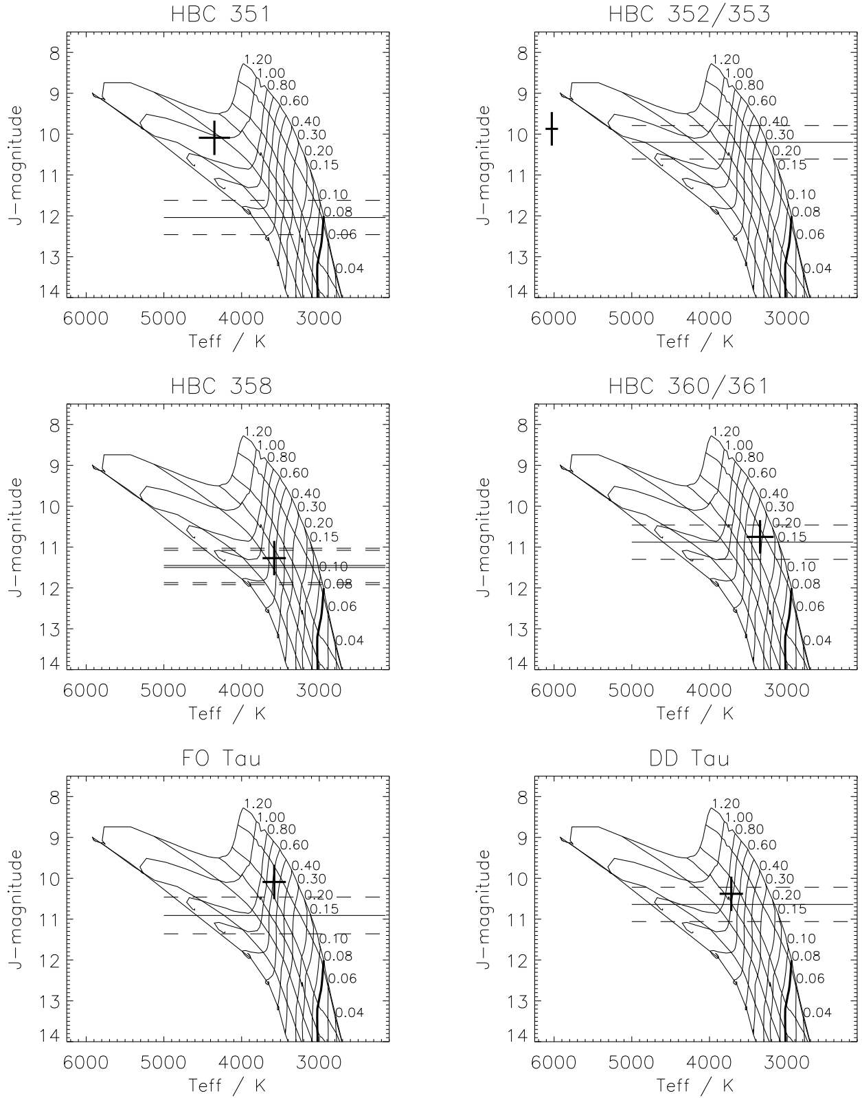
Fig. C.1. Components of T Tauri binary systems placed into the HRD as described in Sect. 5. The cross gives the position of the primary, the horizontal dashed lines give the locus for the companion and the respective error. The PMS model from Baraffe et al. (1998) is also indicated. Evolutionary tracks are plotted for masses of 0.04, 0.06, 0.08 (bold), 0.10, 0.15, 0.20, 0.30, 0.40, 0.50, 0.60, 0.70, 0.80, 1.0 and 1.2 M_{\odot} , the isochrones denote ages of 1, 2, 5, 10, 20, 50 and 90 Myr.
