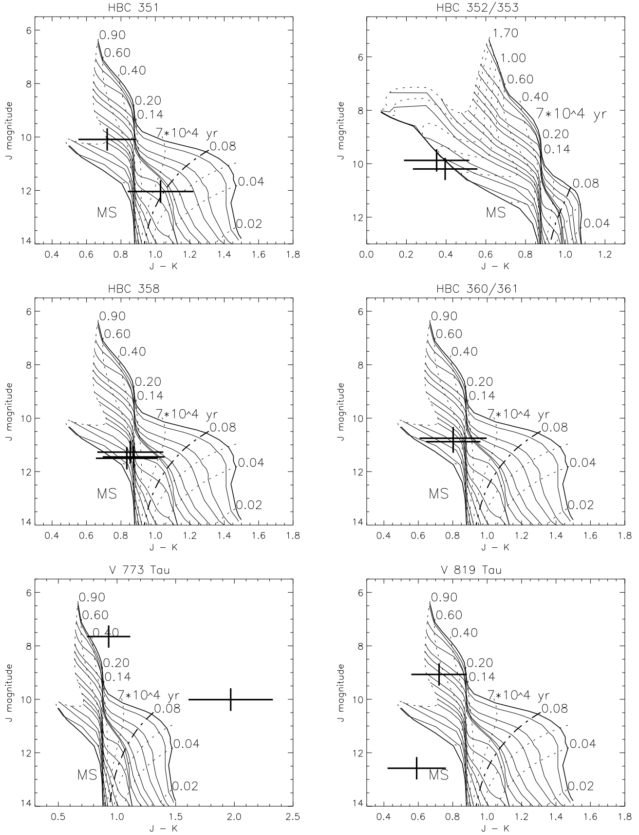
Fig. B.1. Components of WTTS systems placed into NIR color-magnitude diagrams together with the PMS model by D'Antona & Mazzitelli (1998). The dashed lines denote evolutionary tracks for masses from 0.02 to 0.9 M_{\odot} , the solid lines are isochrones for ages 7 \cdot 10^4 , 10^5 , 2 \cdot 10^5 , 3 \cdot 10^5 , 5 \cdot 10^5 , 7 \cdot 10^5 , 10^6 , 2 \cdot 10^6 , 3 \cdot 10^6 , 5 \cdot 10^6 , 7 \cdot 10^6 , 10^7 , 2 \cdot 10^7 , 3 \cdot 10^7 , 5 \cdot 10^7 and 10^8 yr (MS).
