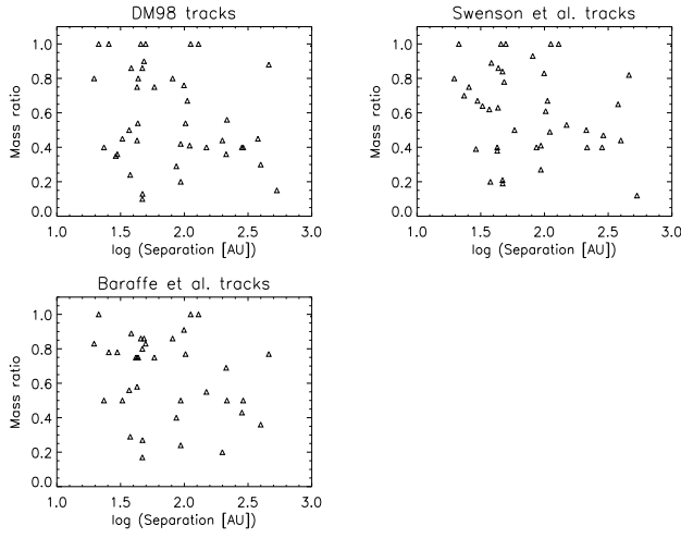
Fig. 8. Distribution of mass ratios as a function of the projected separation for the three sets of PMS models used in this paper.
