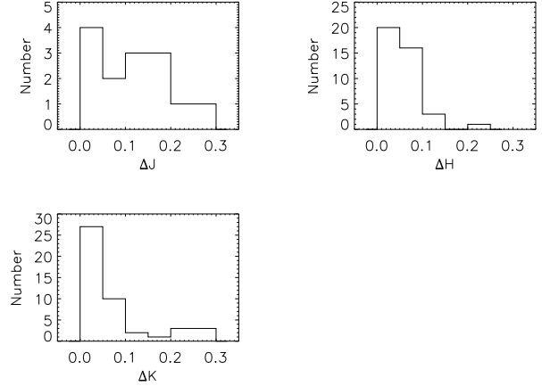
Fig. 2. Distribution of variability amplitudes for components of young binary systems in the NIR spectral bands J, H and K. They contain all of the systems discussed in this paper for which repeated spatially resolved observations in one filter exist (see Table A.1 for our observations and caption of Table A.2 for references to other published data).
